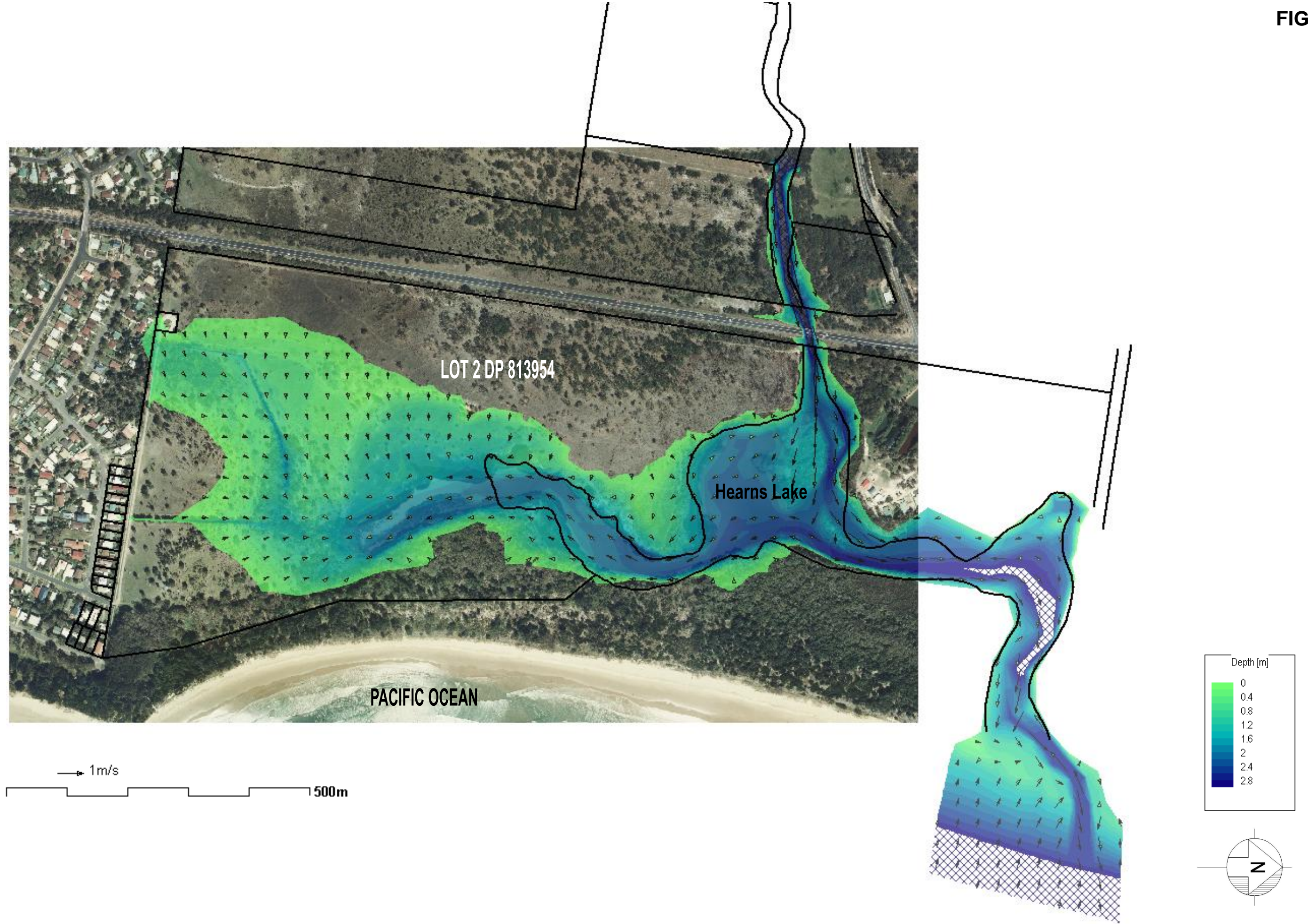
VARIATION IN DEPTH AND VELOCITY OF FLOODWATERS AT THE PEAK OF THE 100 YEAR RECURRENCE FLOOD WITH PROVISION FOR CLIMATE CHANGE
